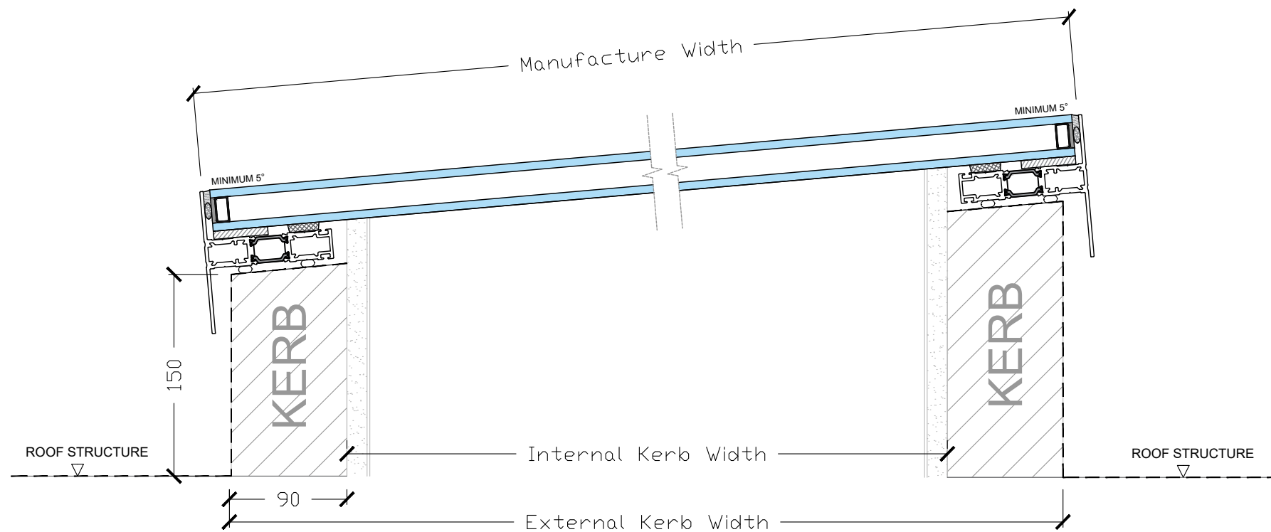
Section Through - Sloped
