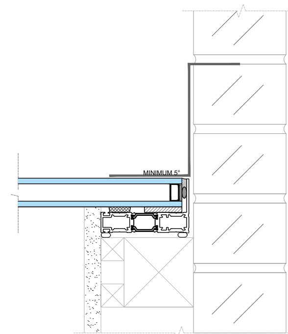
Wall Abutment
